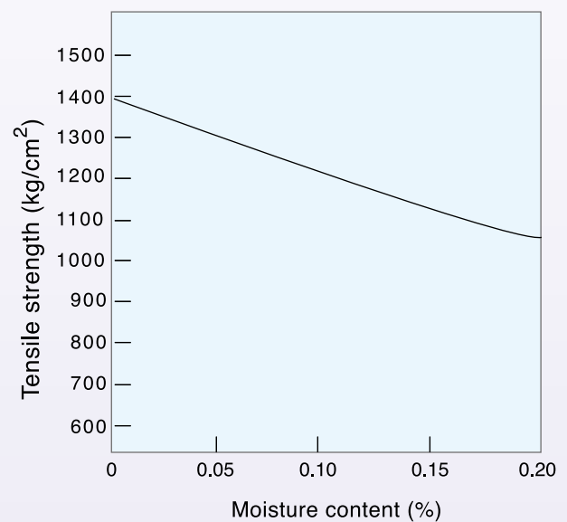
Tensile strength vs. moisture content
